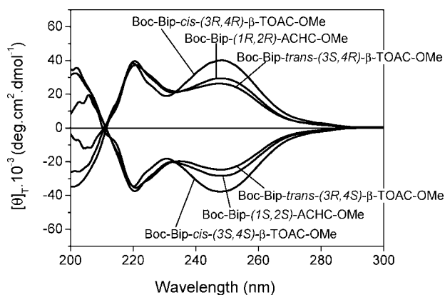
Figure 6. Far-UV CD spectra in MeOH solution of Boc-Bip-(3 S ,4 R )- \beta -TOAC-OMe, Boc-Bip-(3 R ,4 S )- \beta -TOAC-OMe, Boc-Bip-(3 R ,4 R )- \beta -TOAC-OMe, and Boc-Bip-(3 S ,4 S )- \beta -TOAC-OMe, Boc-Bip-(1 R ,2 R )-ACHC-OMe, and Boc-Bip-(1 S ,2 S )-ACHC-OMe. Peptide concentration: 1 mM.
