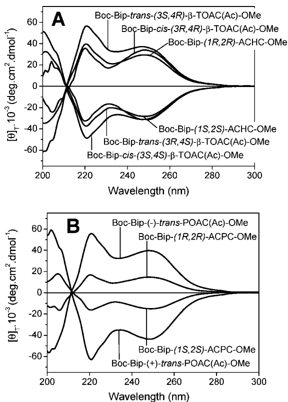
Figure 5. Far-UV CD spectra in MeOH solution of Boc-Bip-(3 S ,4 R )- \beta -TOAC(Ac)-OMe, Boc-Bip-(3 R ,4 S )- \beta -TOAC(Ac)-OMe, Boc-Bip-(3 R ,4 R )- \beta -TOAC(Ac)-OMe, Boc-Bip-(3 S ,4 S )- \beta -TOAC(Ac)-OMe, Boc-Bip-(1 R ,2 R )-ACHC-OMe, and Boc-Bip-(1 S ,2 S )-ACHC-OMe (A), and Boc-Bip-( - )-POAC(Ac)-OMe, Boc-Bip-( + )-POAC(Ac)-OMe, Boc-Bip-(1 R ,2 R )-ACPC-OMe, and Boc-Bip-(1 S ,2 S )-ACPC-OMe (B). 12c Peptide concentration: 1 mM.
