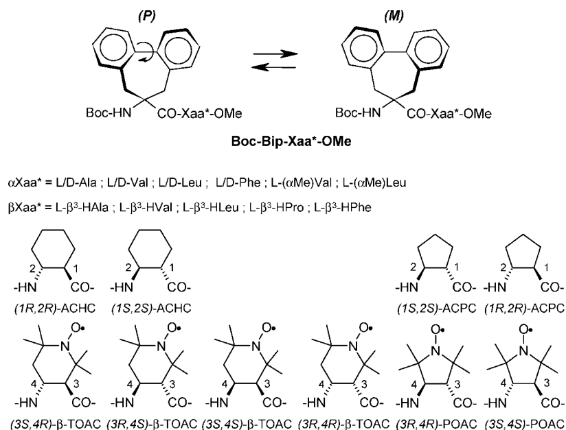
Figure 1. Conformational equilibrium of the Boc-Bip-Xaa*-OMe dipeptides. The abbreviations ACHC, ACPC, \beta -TOAC, and POAC stand for 2-amino-cyclohexanecarboxylic acid, 2-amino-cyclopentanecarboxylic acid, 4-amino-1-oxyl-2,2,6,6-tetramethylpiperidine-3-carboxylic acid, and 4-amino-1-oxyl-2,2,5,5-tetramethylpyrrolidine-3-carboxylic acid, respectively.
